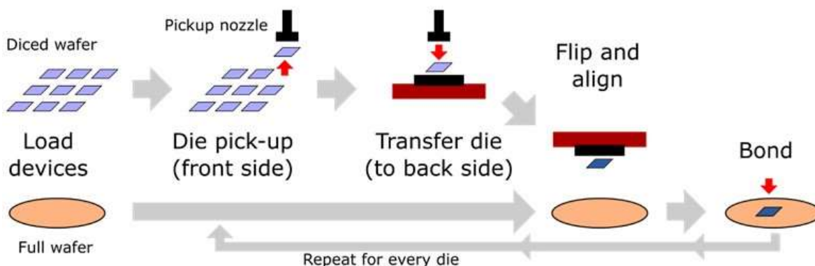
Figure 11: Schematic of the Die-to-Wafer Micro-bump Bonding Process
