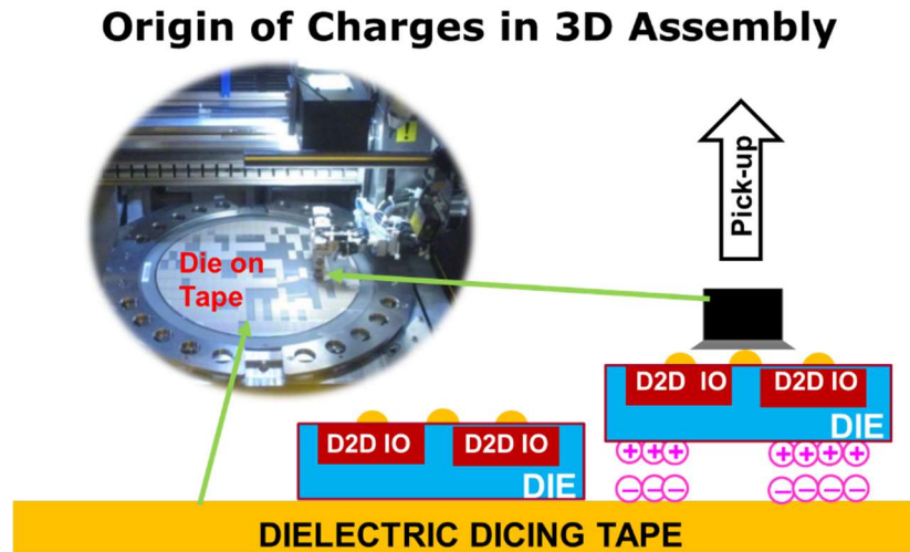
Figure 9: Charging Process During Die Assembly
